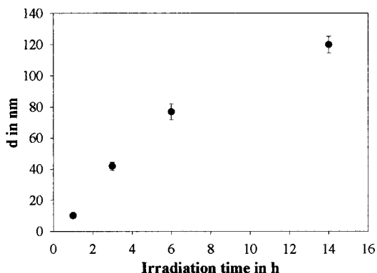
Figure 5: Dependence of the polymer layer thickness on the irradiation time at \lambda_{\text{max}} = 350 \text{ nm} ; (●) series of individually prepared samples cleaned by exhaustive washing with toluene (layer thickness was measured by AFM; values are averaged values calculated from six measurements of individual spots on each sample; error bars reflect the standard deviation).
