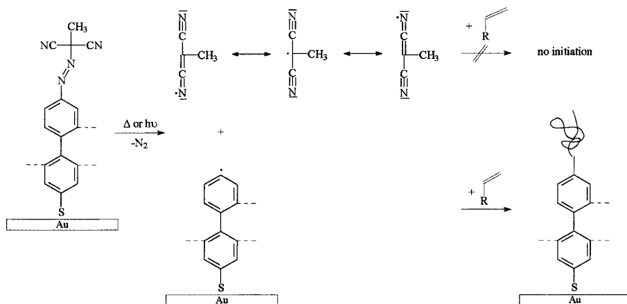
Figure 1: Surface-bond initiator SAM used for the thermal and photochemical SIP.
